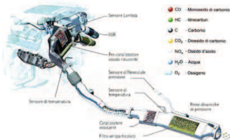
Fig.2 - SISTEMA CDPF (CAT PARTICULATE FILTER)
